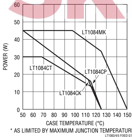
LT1084 Maximum Power Dissipation*
